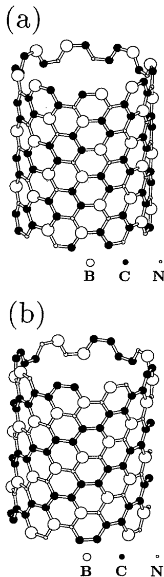
FIG. 2. The BC_2N (4,4) tubules obtained by rolling (a) type-I sheets and (b) type-II sheets. The vertical direction is parallel to the tubule axes. Some atoms in the back sides are not shown to avoid complexity. The chiral alignments of C, B, and N atoms are seen in these structures.
