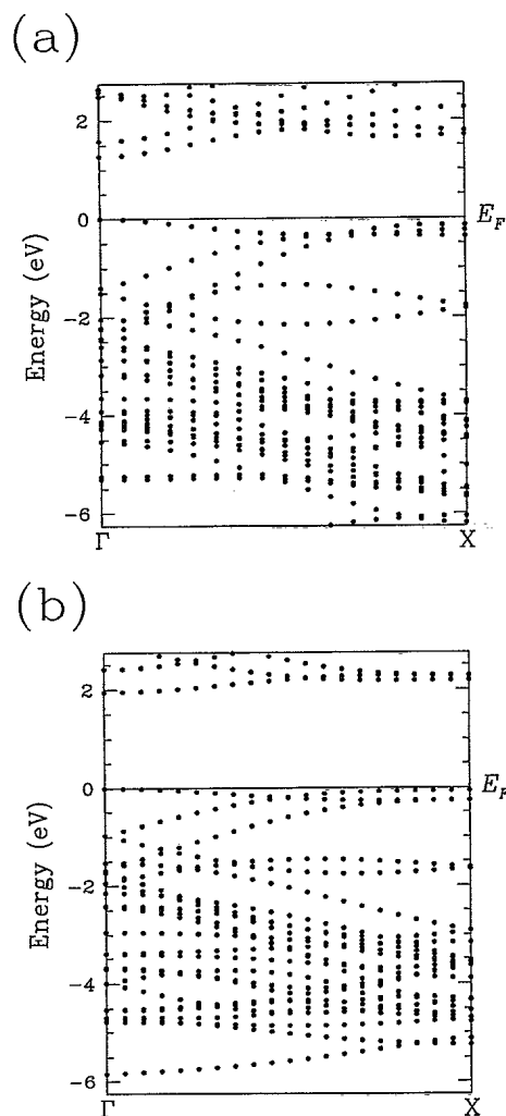
FIG. 3. Energy band structures of type-II (2,2) tubules obtained by (a) LDA calculations and (b) sp^3s^* nearest-neighbor TB calculations.
