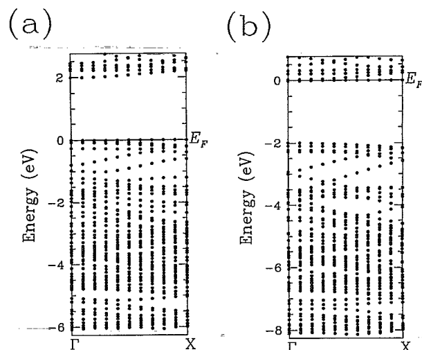
FIG. 4. Energy band structures of the type-II (2,2) tubules having an impurity C atom (a) on a N site and (b) on a B site obtained by the sp^3s^* nearest-neighbor TB calculation. The locations of E_F here correspond to the locations of the impurity-induced levels. The assumed periodic boundaries are twice as those of the (2,2) tubules so the first Brillouin zones are half of those in Fig. 3.
